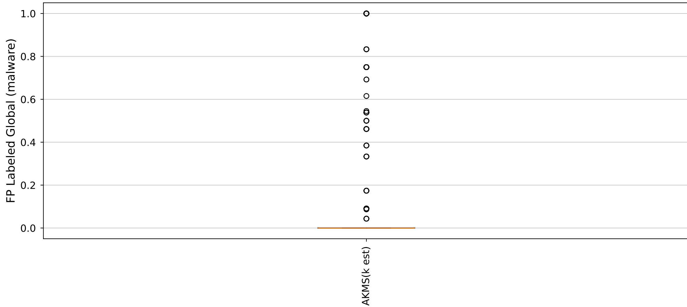
YARA Rules FP Labeled Global (malware) Distribution (Cluster0_Size134 dataset)
